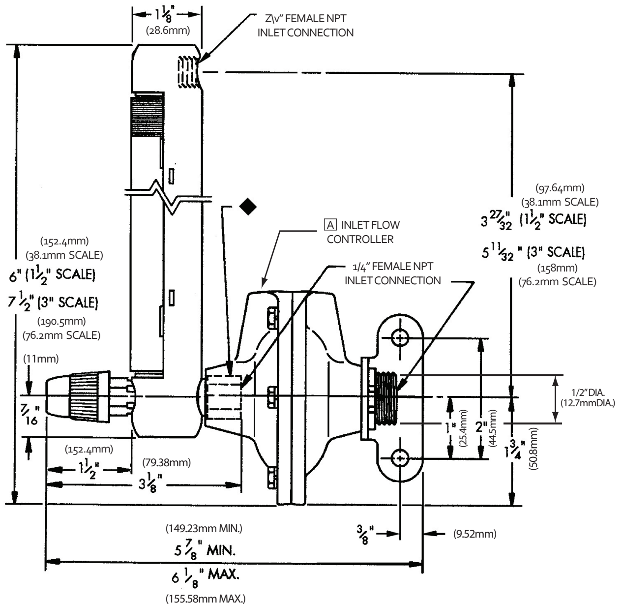
Purge Meter With Control Valve And Inlet Flow Controller
